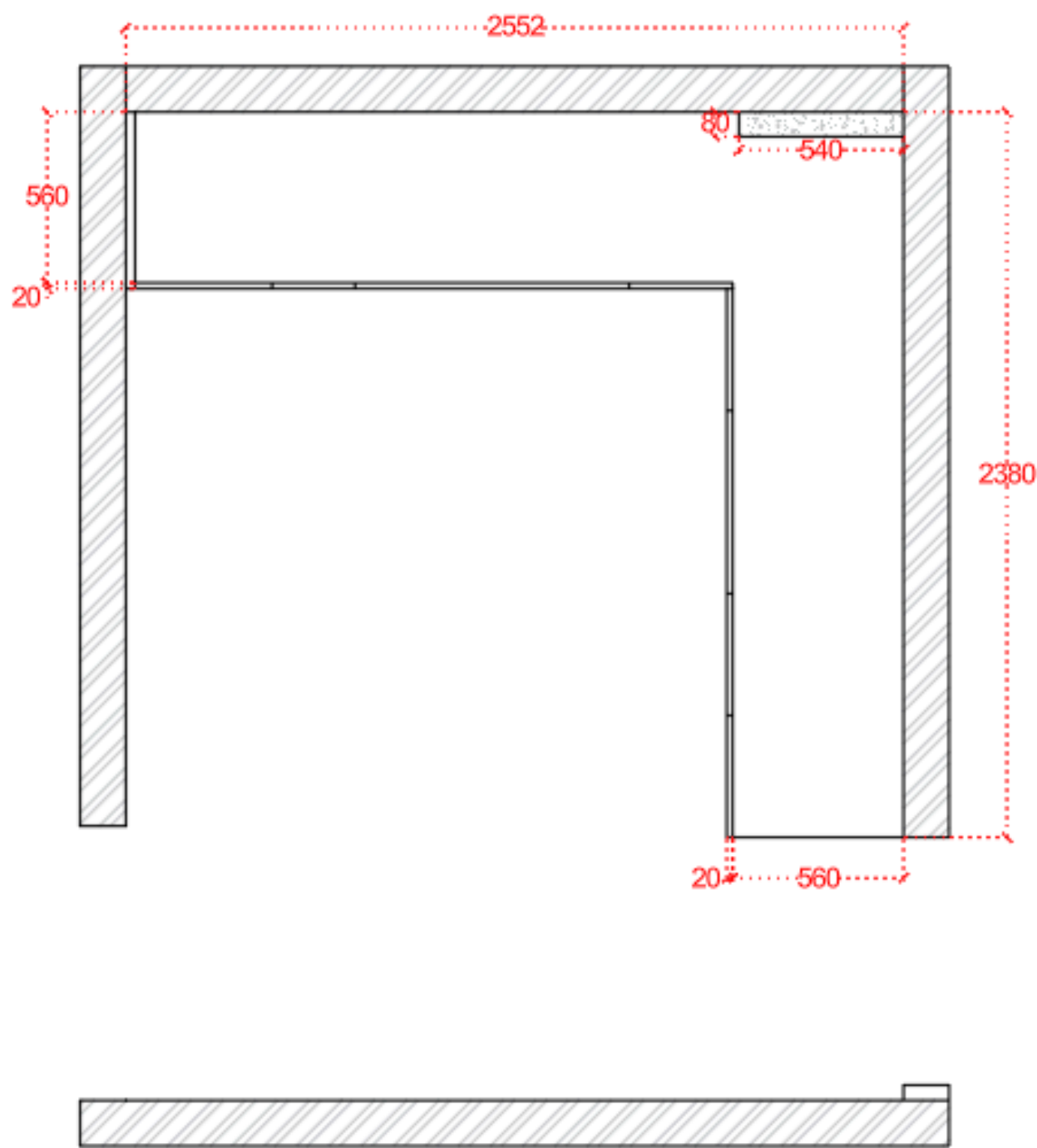
KITCHEN BASE UNIT TOP VIEW
