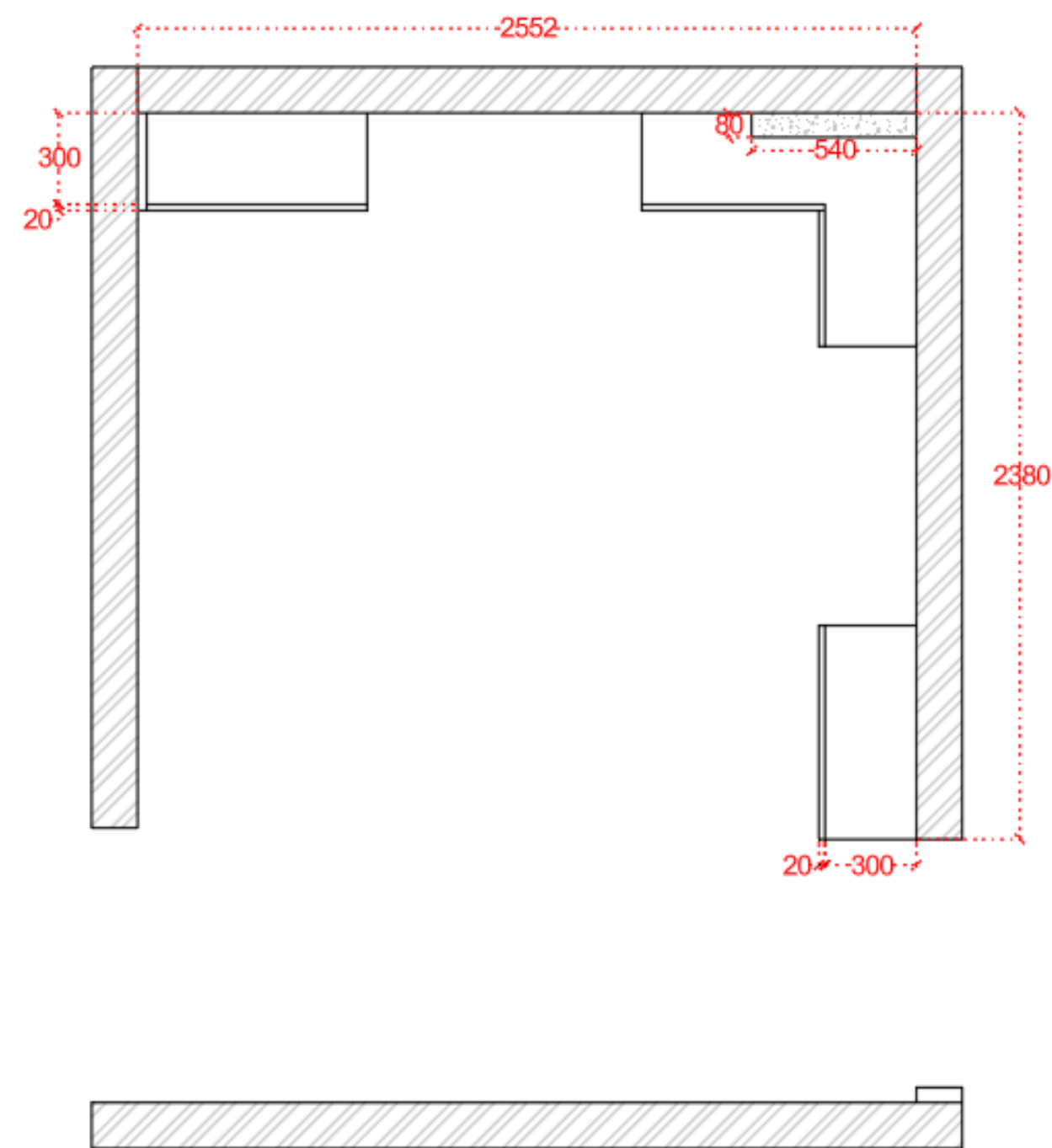
KITCHEN WALL UNIT TOP VIEW
